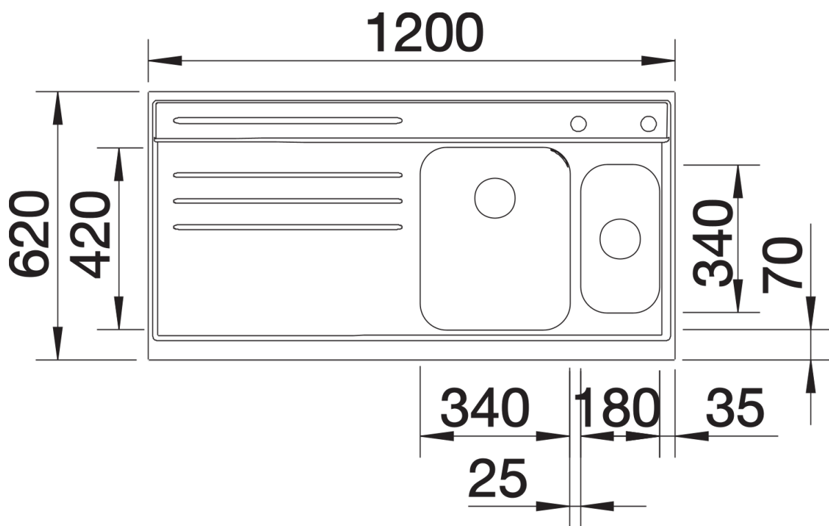
Top view
