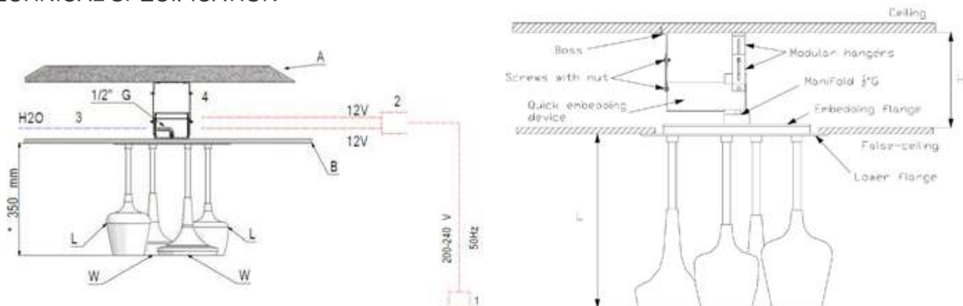
Front View- Installation of Shower Heads & Water and Lighting Connections
