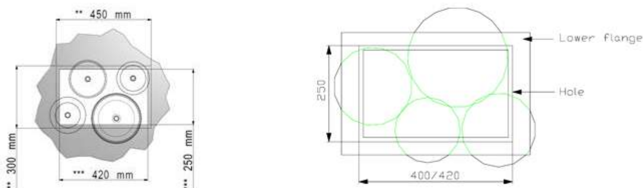
Top View- Fixing Plate Dimensions
